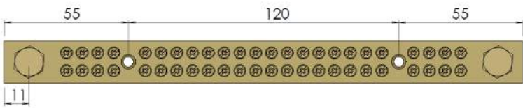
TYPICAL 24 POLE/WAY WITH 120mm MOUNTING CENTRES
